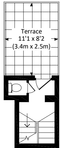
FIRST FLOOR MEZZANINE
