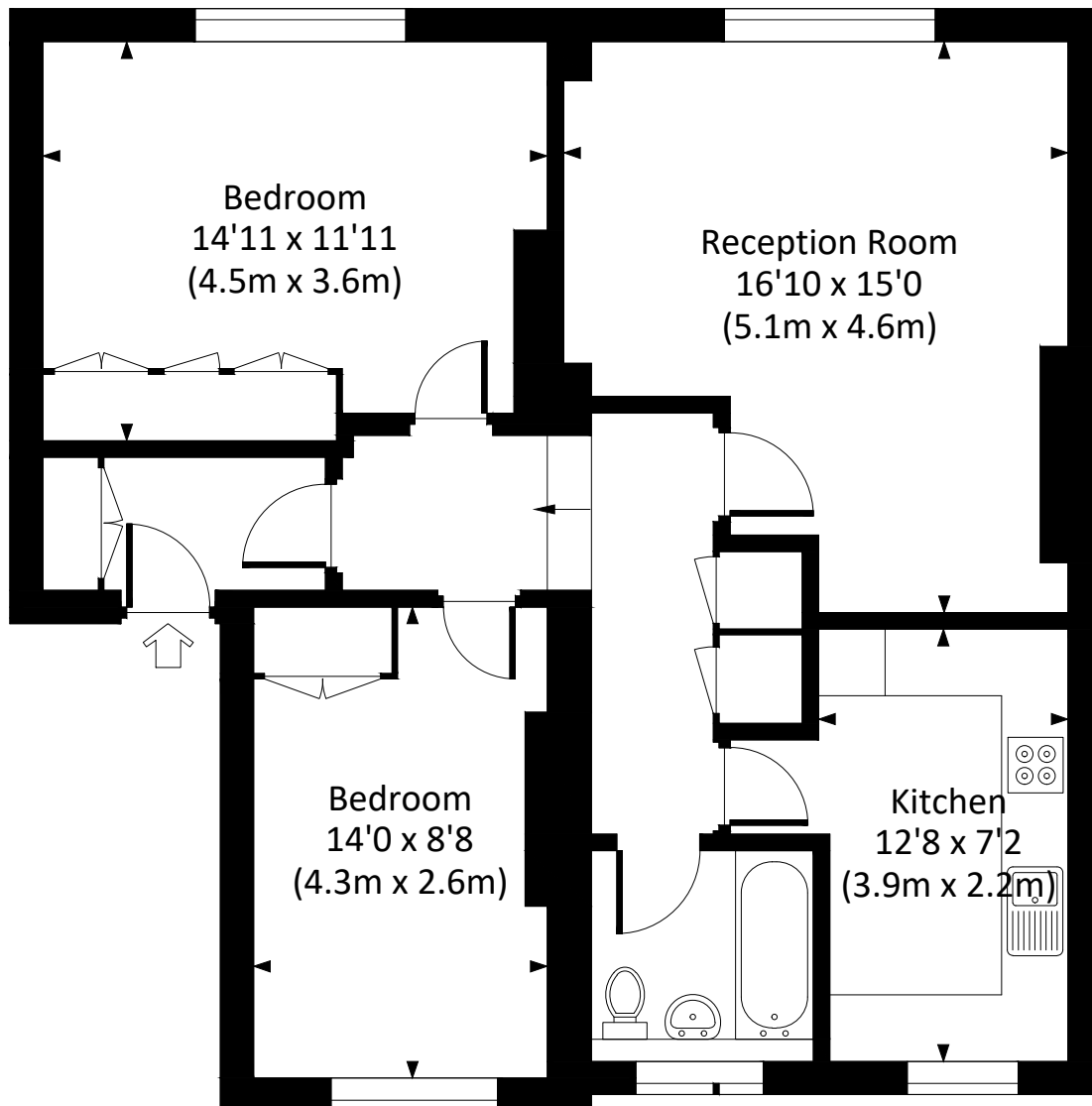
FIRST FLOOR
