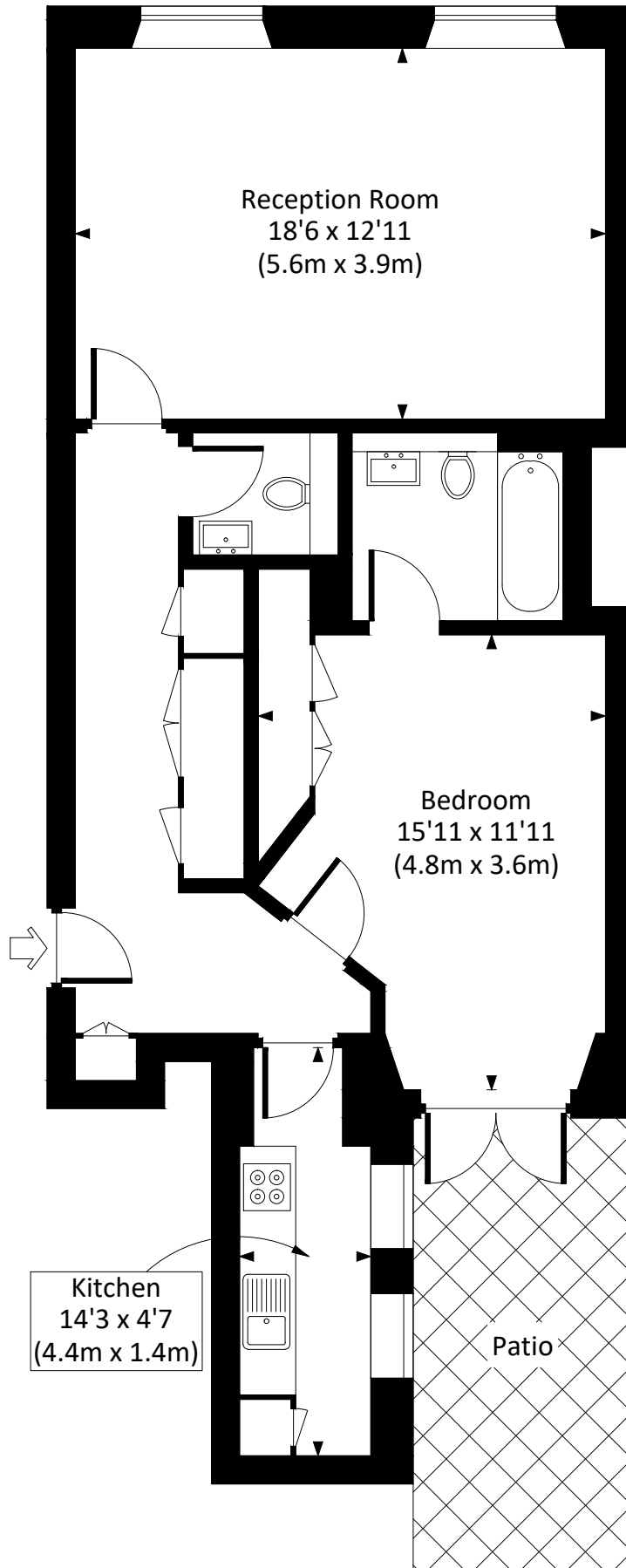
GROUND FLOOR
