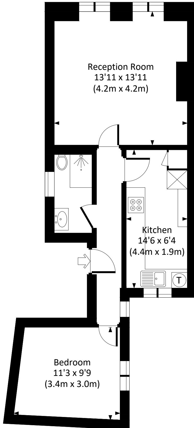
FIRST FLOOR
