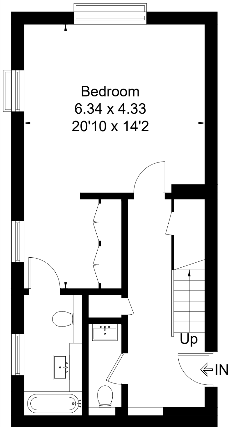
Fourth Floor
